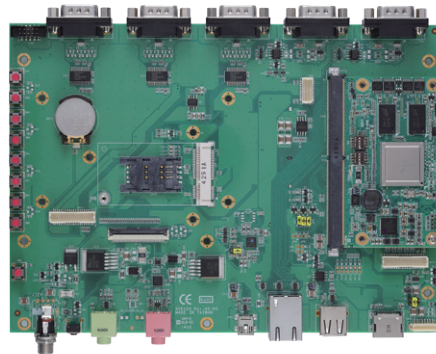
▲ SCM120-120-EVK
